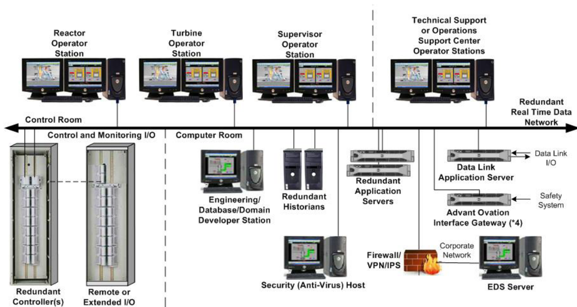
I&C systems platform
