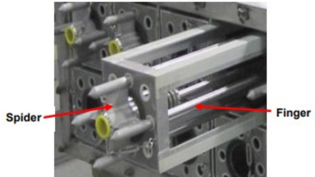
16x16 Five Finger CEA in a shipping container cradle
