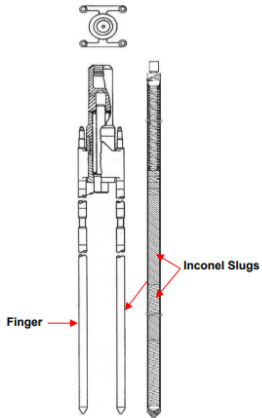
System 80 Part-Strength CEA
